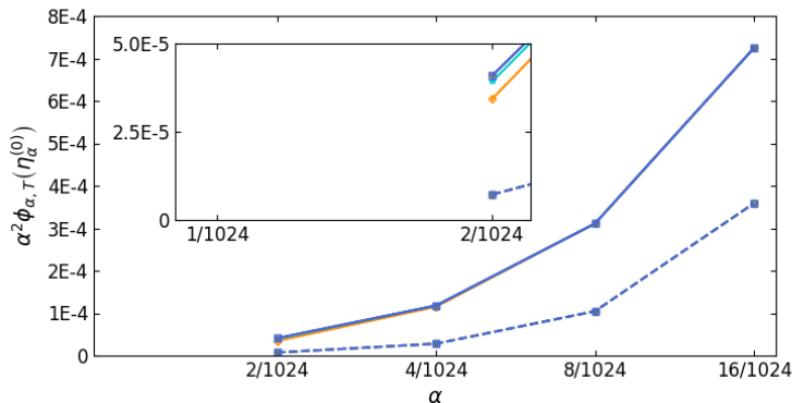
Figure: Results for T = 3 (dotted line) and for T = 5 (solid line). Results from runs performed at different resolutions are displayed together: 128^3 (orange plus), 256^3 (cyan star), 512^3 (brown triangles), and 1024^3 (blue squares).
