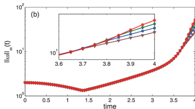
Figure: (Bustamente et al. 2012, Fig. 1b) Maximum of vorticity \|\omega(\cdot, t)\|_\infty . Results from runs performed at different resolutions are displayed together: 512^3 (brown triangles), 1024^3 (blue squares), 2048^3 (green diamonds), and 4096^3 (red circles).
